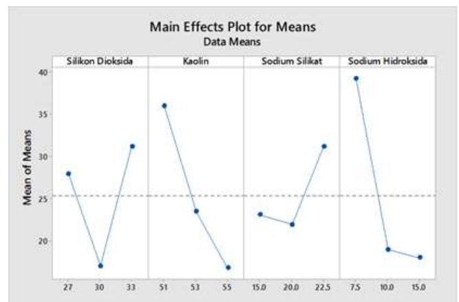
Figure 5: Effect plot for Means
