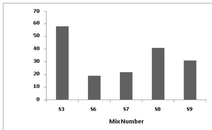
Figure 7: The average flexural strength of 5 optimum samples
