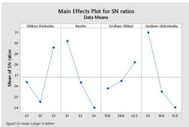
Figure 4: Effect plot for SN ratios
